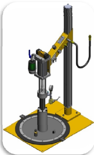
Drum pump P100/113-2L Delivery/double stroke 113 cm 3 Pressure ratio 21 : 1
