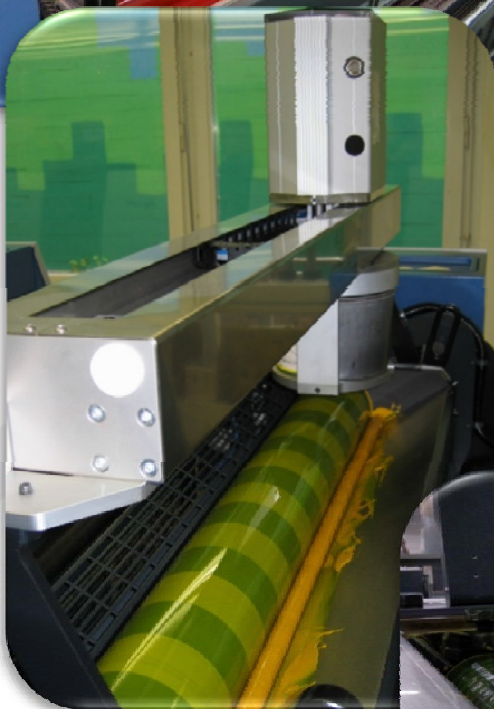
Automatic ink filling of the ink fountains out of standard 2,5kg cans. Version for UV plastic cans is also available.
