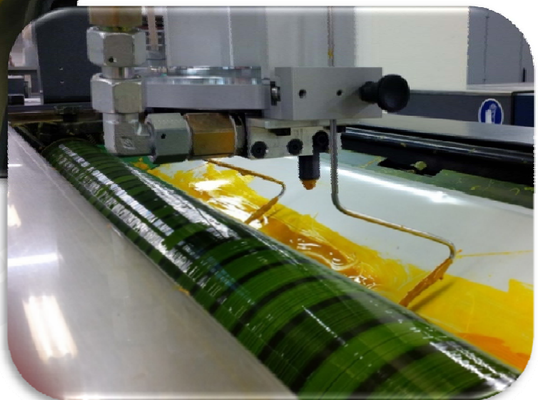
Automatic ink filling of the ink fountains out of standard 2,5kg cans. Version for UV plastic cans is also available.
