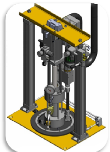
Pail can pump P100/150-25H/L/UV Delivery/double stroke 113 cm 3 Pressure ratio 8 : 1
