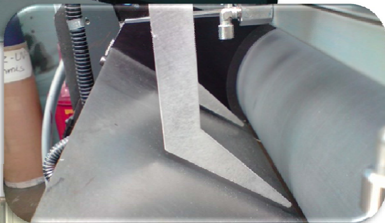
Ink agitator BIA-PSH with double scraper blade
