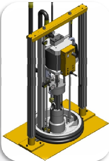
Drum pump P200/329-2L/DH Delivery/double stroke 329 cm 3 Pressure ratio 30 : 1
