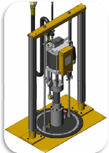
Drum pump P200/329-2L Delivery/double stroke 329 cm 3 Pressure ratio 30 : 1
