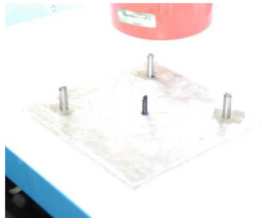
Melting punch device for plastic cans
