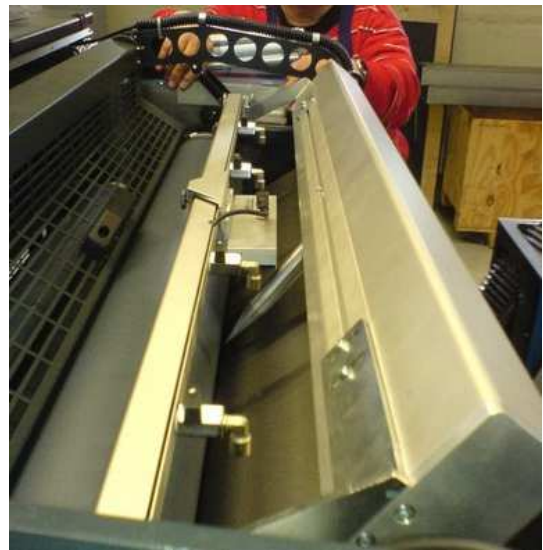
Pneumatically driven ink agitator BIA with rotating cone
