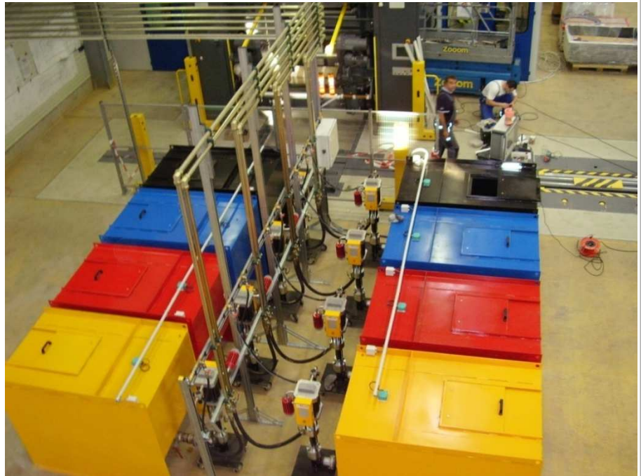
Pump stations installed with 1500 kgBase container
