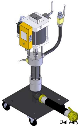
Containerpump P250/656-1/PLC Delivery rate / cycle 656 cm 3 Pressure ratio 23 : 1
