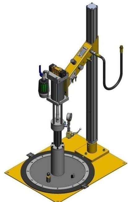
200 kg Fasspump P100/113-2L Delivery rate / cycle 113 cm 3 Pressure ratio 21 : 1
