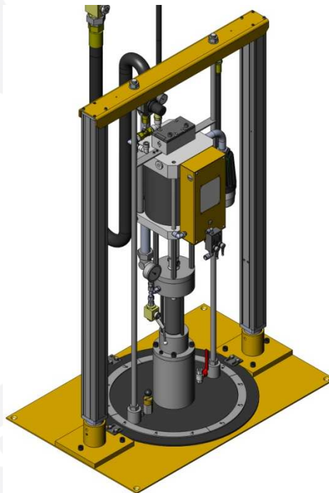
200 kg Fasspump P200/329-2L Delivery rate / cycle 329 cm 3 Pressure ratio 30 : 1
